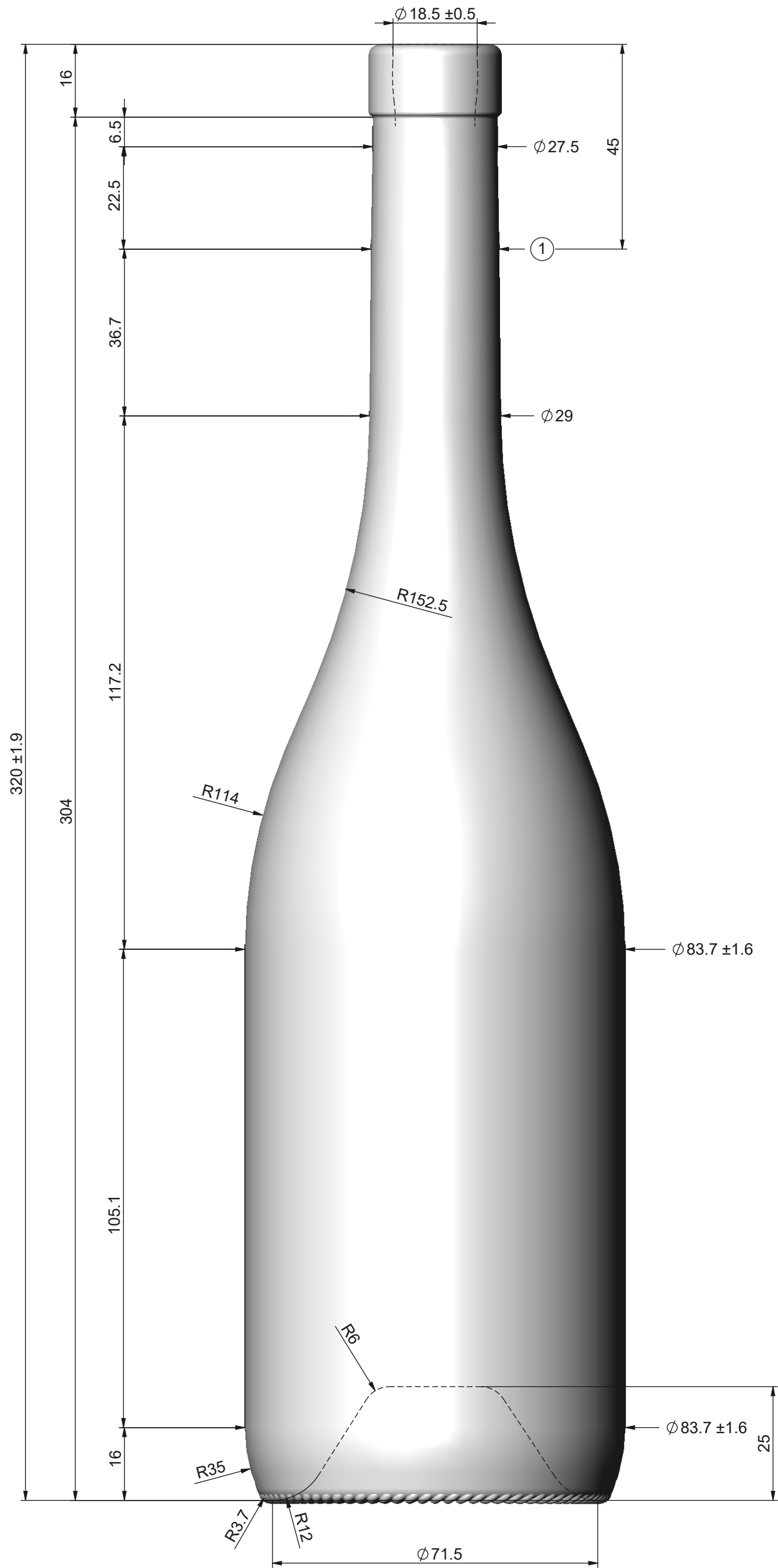
FRONT VIEW
